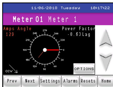
Single Phase Phasor screen
