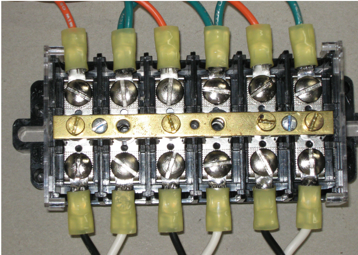
Figure 4.7: EI SB-6TC with All CTs Shorted Properly
