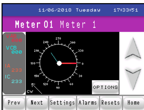
2 CT Delta Phasor screen
