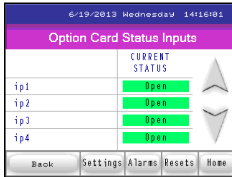
Option Card Status Inputs screen
