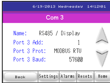
Com 3 Settings for MP200 Unit
