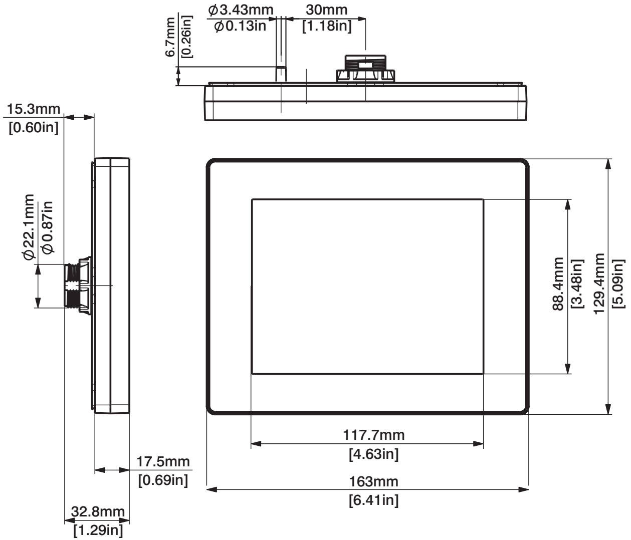
Figure 10.4: MDLN Dimensions
