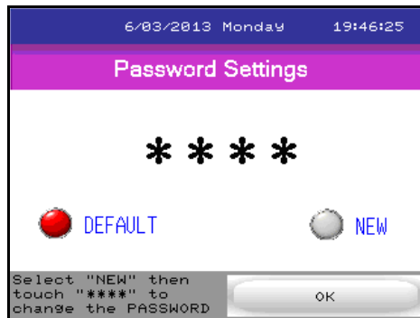
Password screen
