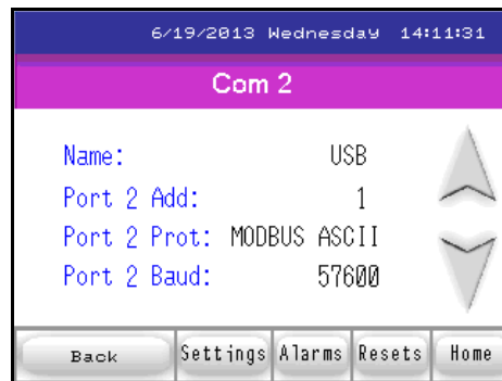
Com 2 Settings for MP200 Unit
