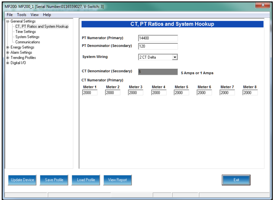
MP200 Unit with Three Phase Configuration - MP200-Y: 2 CT Delta
