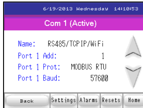
Com 1 Settings for MP200 Unit
