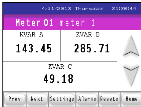
Three Phase VAR per Phase screen (Wye configuration only, not Delta configuration)
