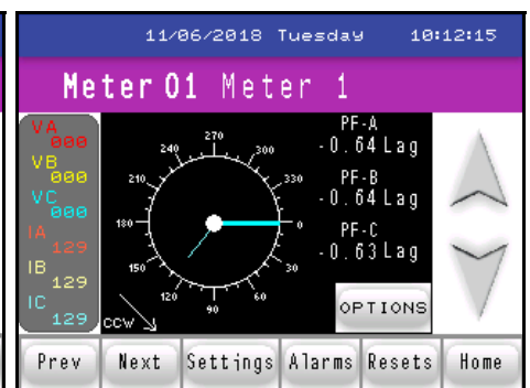
Three Phase Phasor screen
