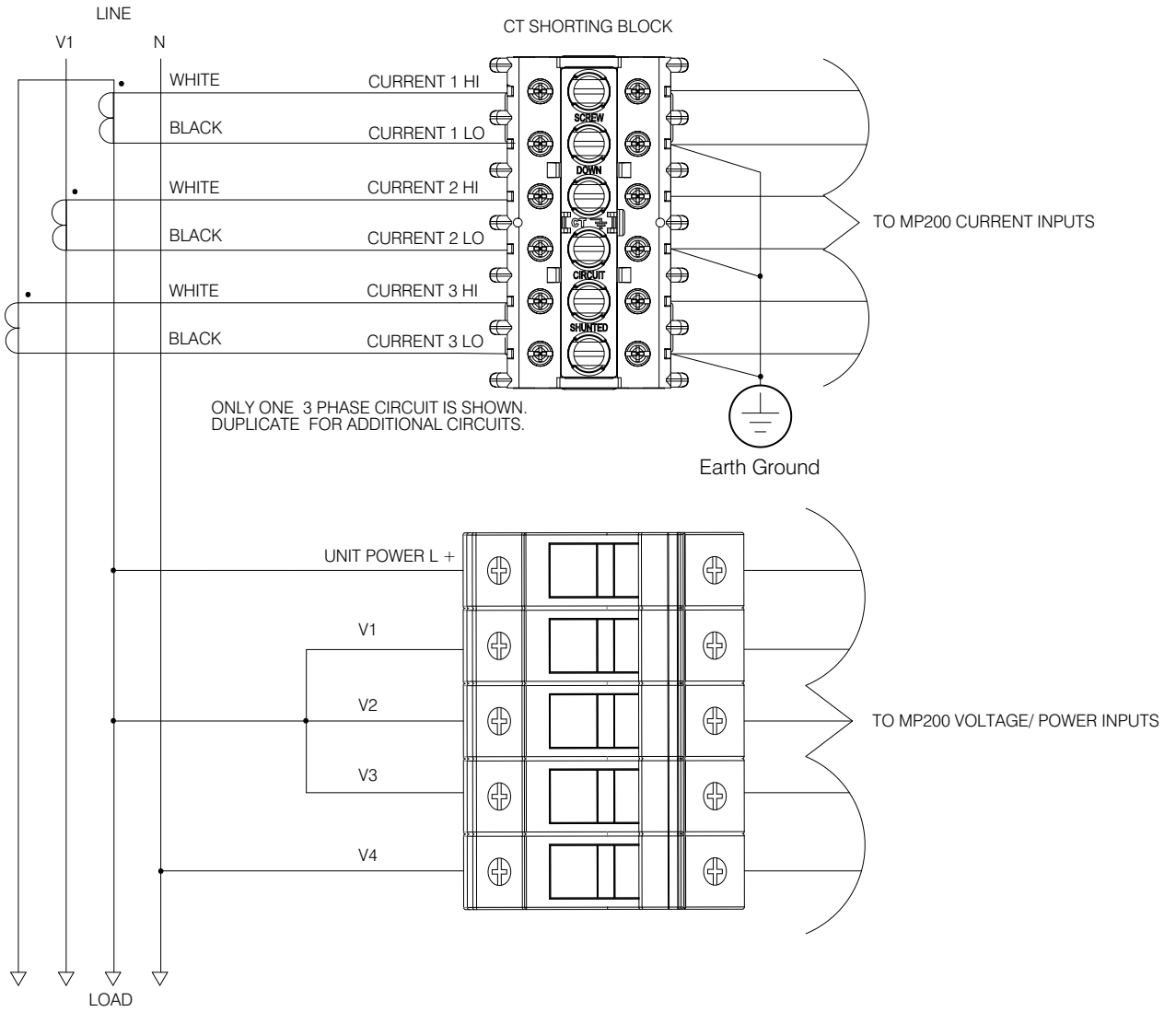
Figure 3.3: MP200-S Single Phase 2 Wire Wiring Diagram
