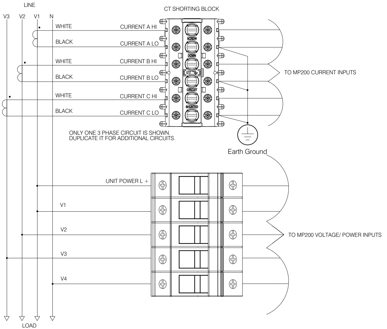
Figure 3.2: MP200-Y Three Phase Wiring Diagram
