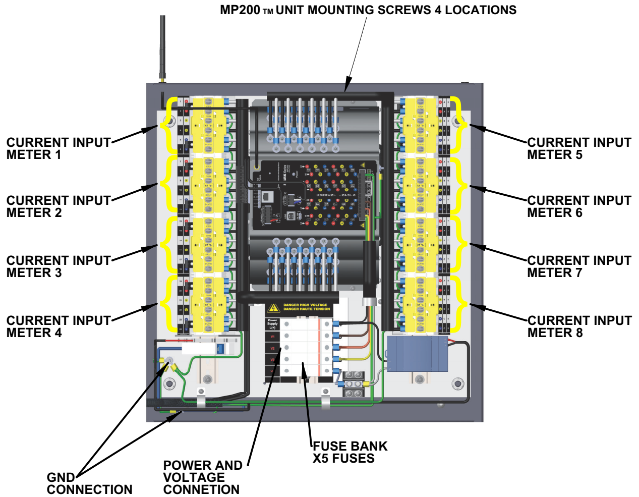
Figure A.3: MP200-Y in Enclosure Location of Fuses, Current Leads, Connectors, Mounting Screws
