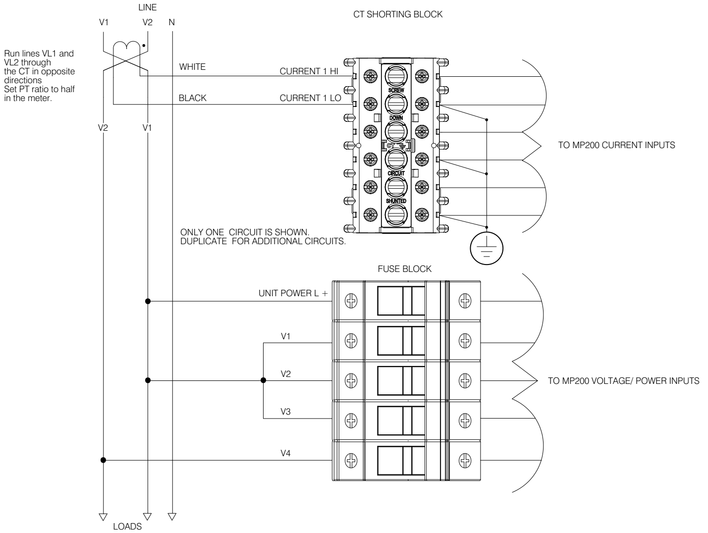
Figure 3.4: MP200-S Single-Phase 3 Wire Wiring Diagram
