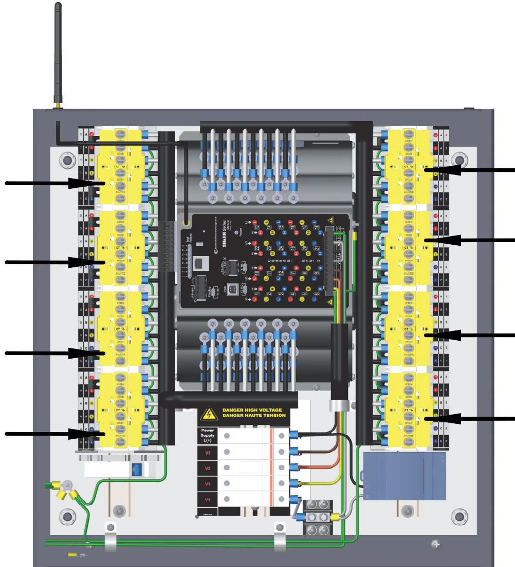
Figure A.1: CT/Shorting Block Location
