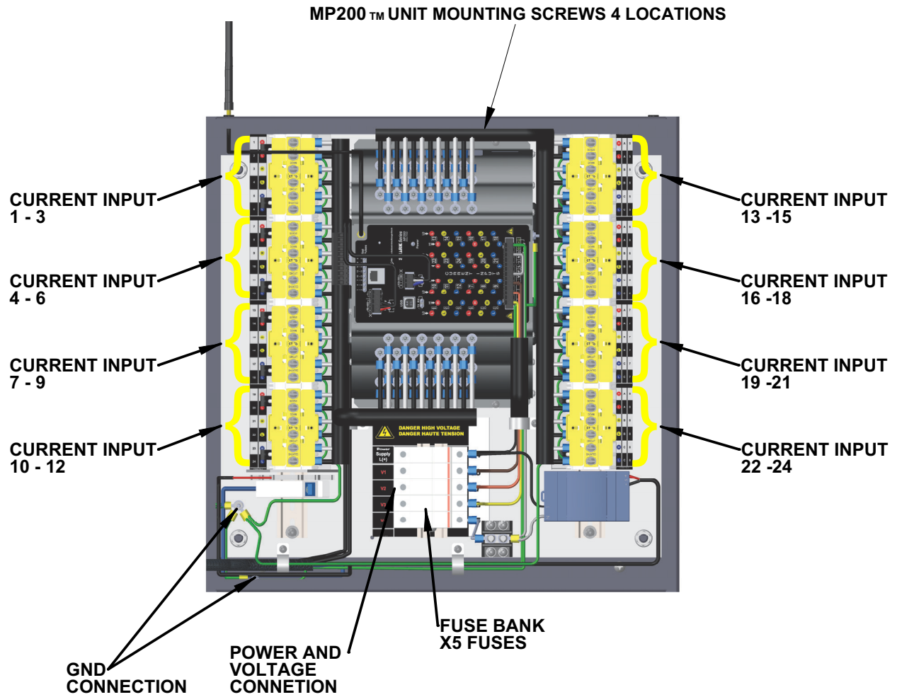
Figure A.4: MP200-S in Enclosure Location of Fuses, Current Leads, Connectors, Mounting Screws
