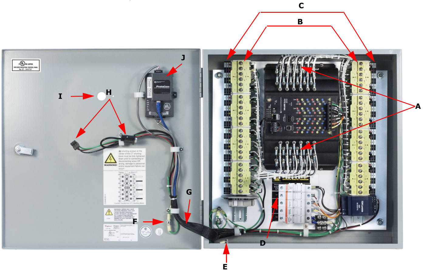
Figure 2.1: MP200™ in Enclosure as Shipped
